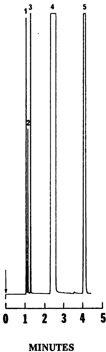
Figure 2. Chromatogram of a reaction mixture with 0.050 ml TEOF reaction solution and 0.50 ml DMF containing 0.187% H 2 O. Peak assignment: 1, ethanol; 2, ethyl formate; 3, methylpentane; 4, DMF; 5, TEOF. Other conditions are given in the text
